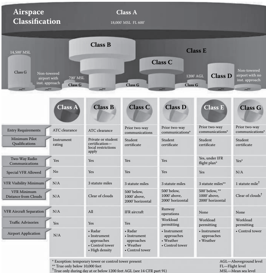
FIGURE 4.3 Airspace is divided into six separate categories.
